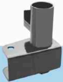
CODE NO. : SHBF 1112 PART NAME : REAR SPRING FRONT HANGER SINGLE SUPPORT (RH) VEHICLE : MAHINDRA MAXX
